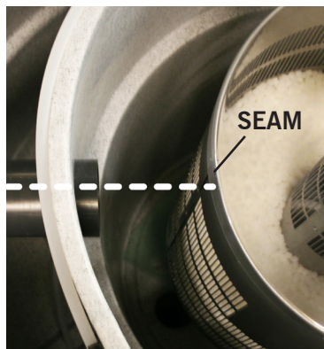
Figure 16. Align the Eazy seam to the centre of the overflow pipe.
